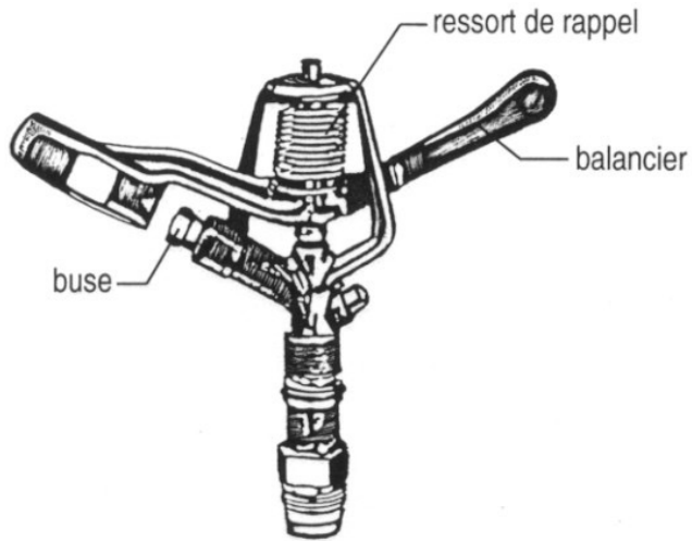
Medium pressure (sprinkler)
